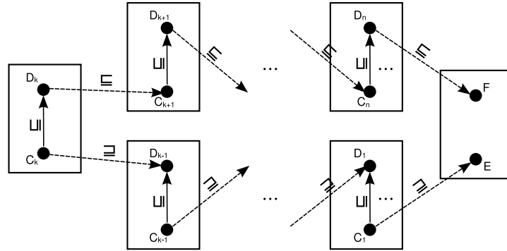
Fig. 3. Depiction of the distributed TBox from Theorem 4. Local subsumption is indicated by solid arrows and bridge rules are indicated by dashed arrows.
