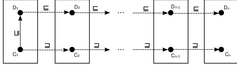
Fig. 2. Depiction of the distributed TBox from Theorem 2. Local subsumption is indicated by solid arrows and bridge rules are indicated by dashed arrows.
