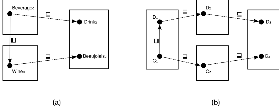
Fig. 1. Depiction of two distributed ontologies of Examples 2, 3 (a), and Example 4 (b). Local subsumption is indicated by solid arrows and bridge rules are indicated by dashed arrows.
