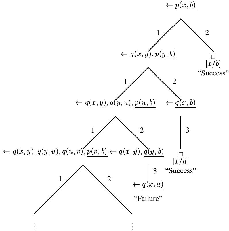
Figure 1. An infinite SLD-Tree
