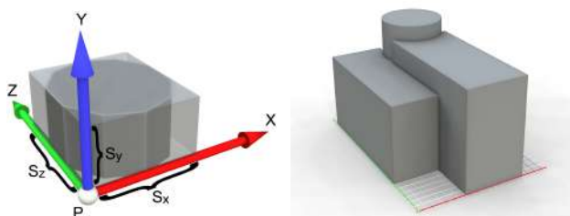
Figure 3: Left: The scope of a shape. The point P , together with the three axis X , Y , and Z and a size S define a box in space that contains the shape. Right: A simple building mass model composed of three shape primitives.
